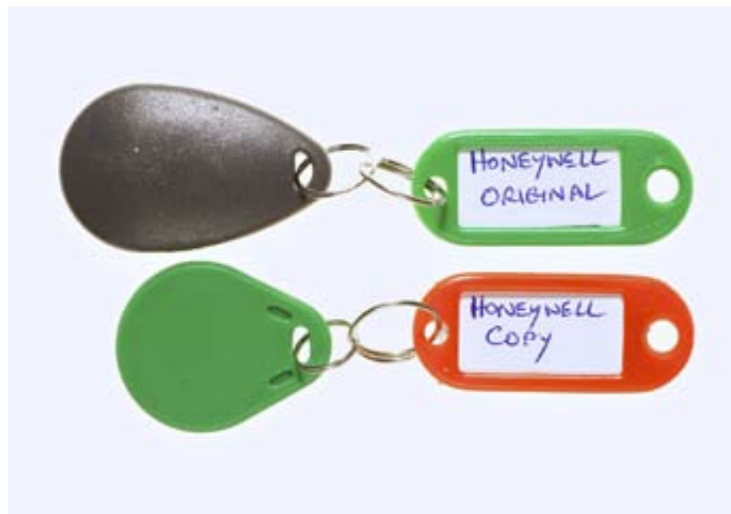
Honeywell – 125 kHz RFID. Galaxy Systems, part ref: YX0-0020
