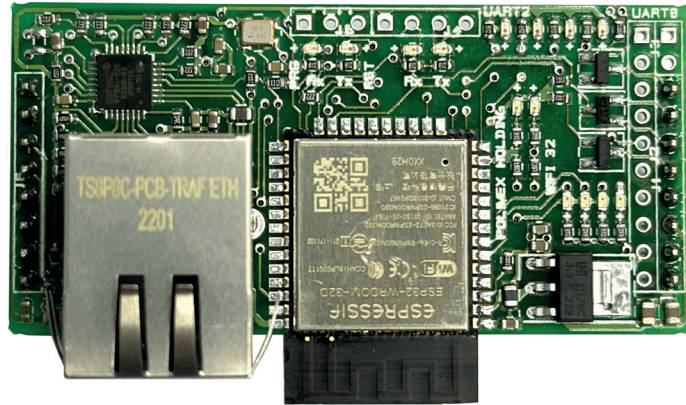
Ethernet & Wi-Fi module for Icon series controllers
